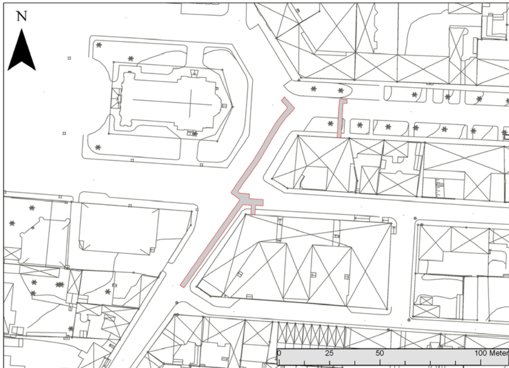
Figur 2.Schaktplan.
